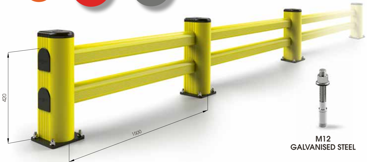
LM 1500x500 MODULAR Equipped with accessories
